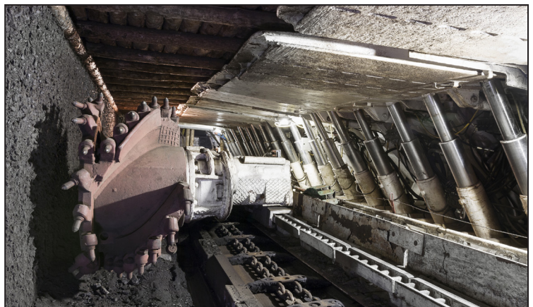
Coal is cut from the coalface by the shearer, while hydraulic jacks support the roof.
